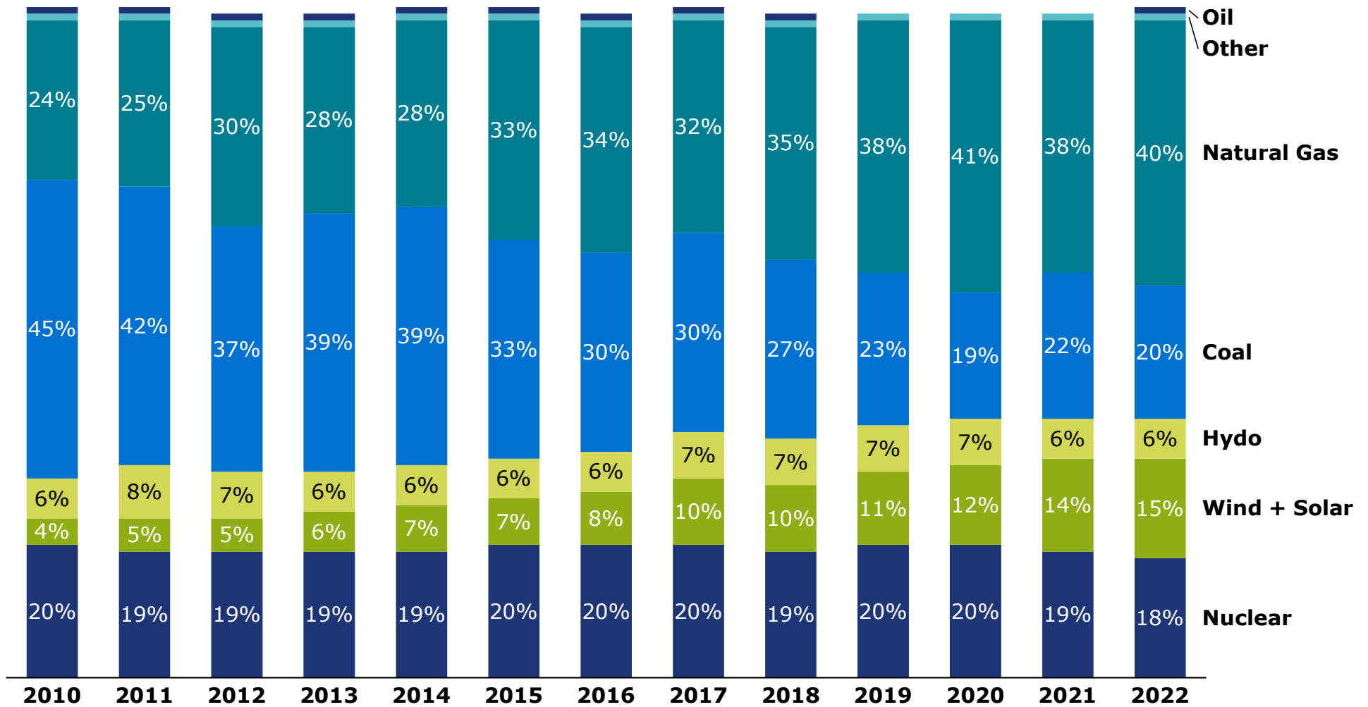
Annual Percent of electric generation by source
